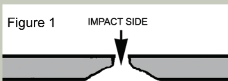
Figure 1 IMPACT SIDE The side of the slate opposite the impact side breaks out and leaves a crater. The impact side has a clean edge and no crater.
